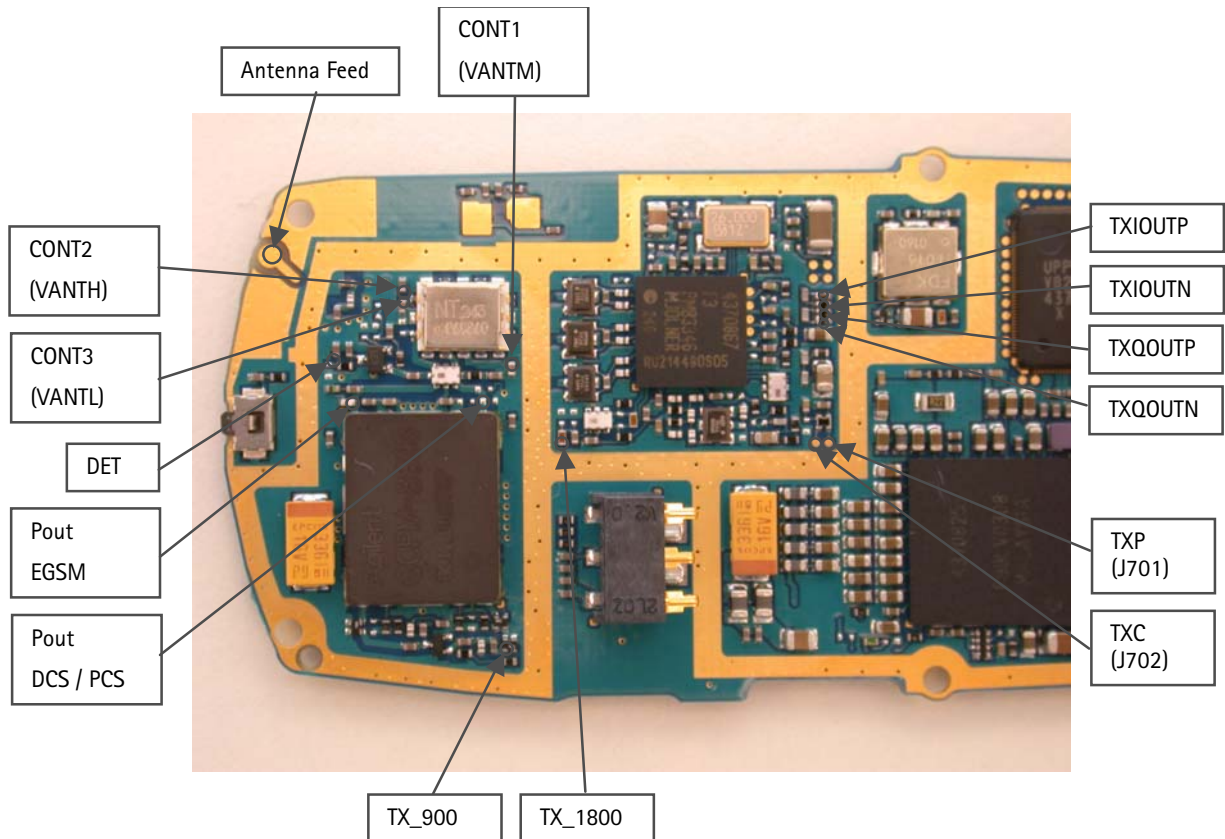
Figure 3: Test points of the transmitter
