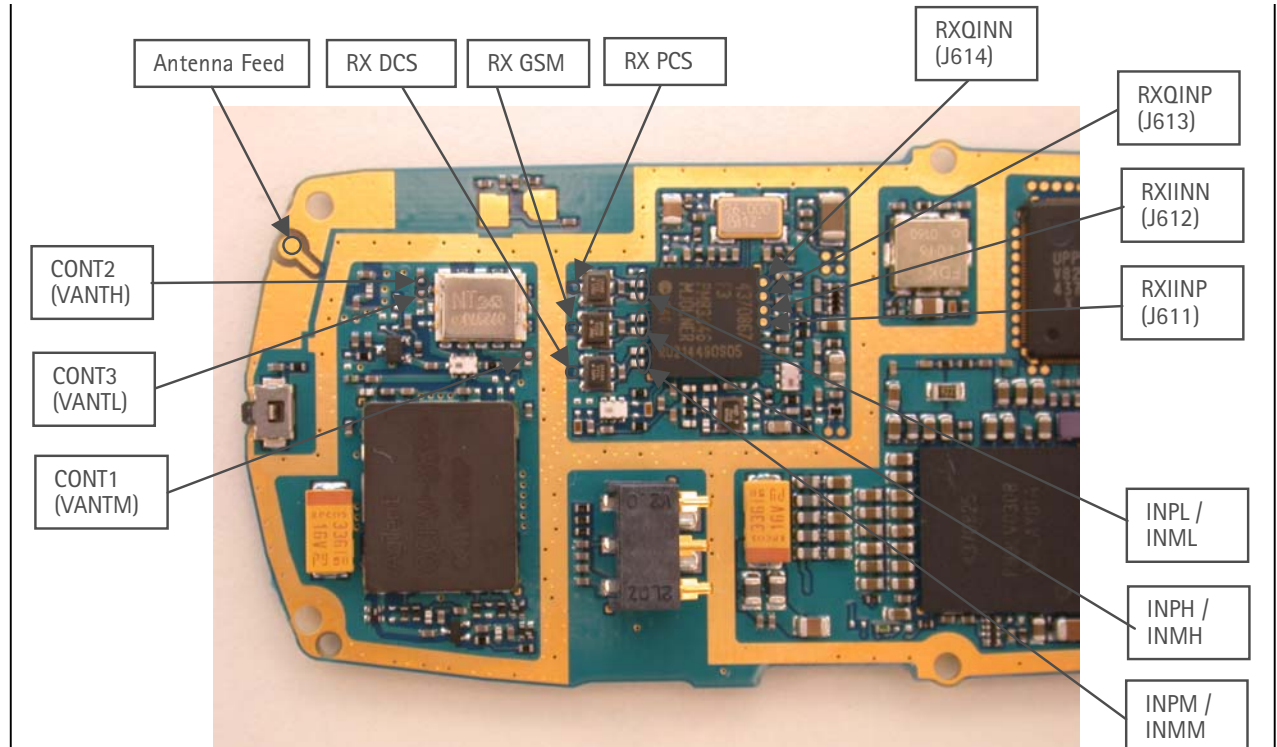
Figure 2: Test points of the receiver
