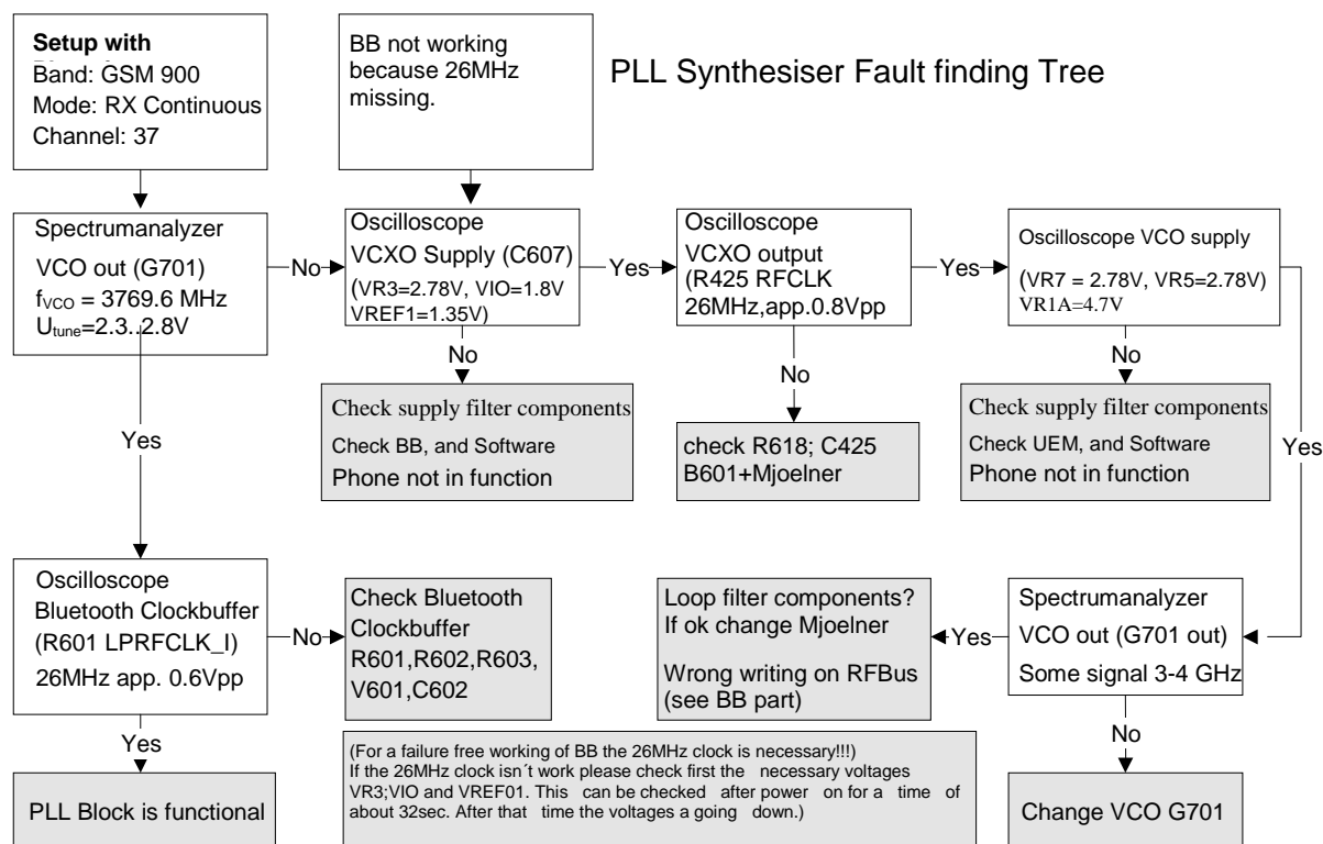
Figure 10: PLL Sythesizer Fault Finding Chart
